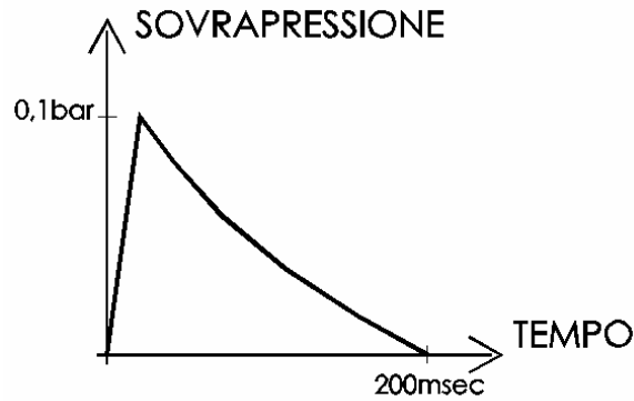
Figure 3. Overpressure versus time diagram
